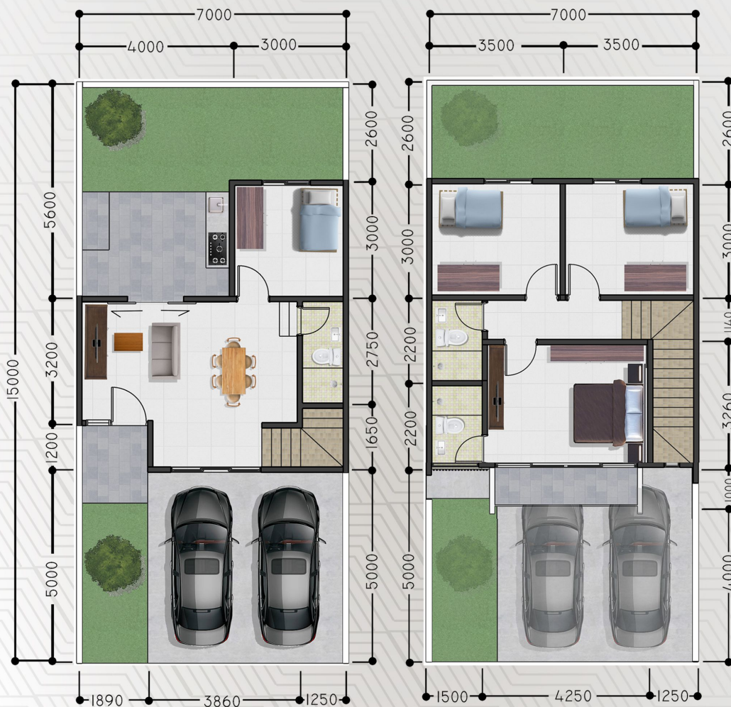
DENAH LT. 1
