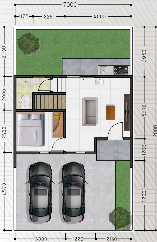
DENAH LT. 1
