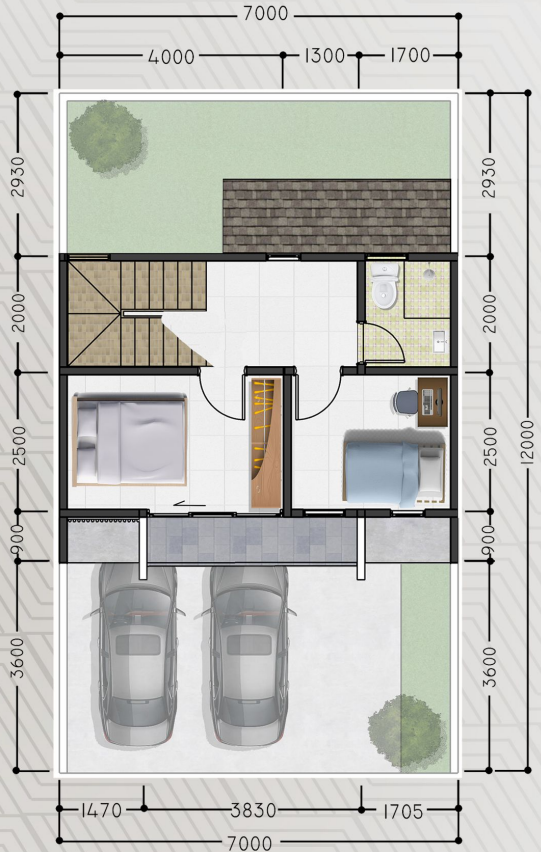
DENAH LT. 2
